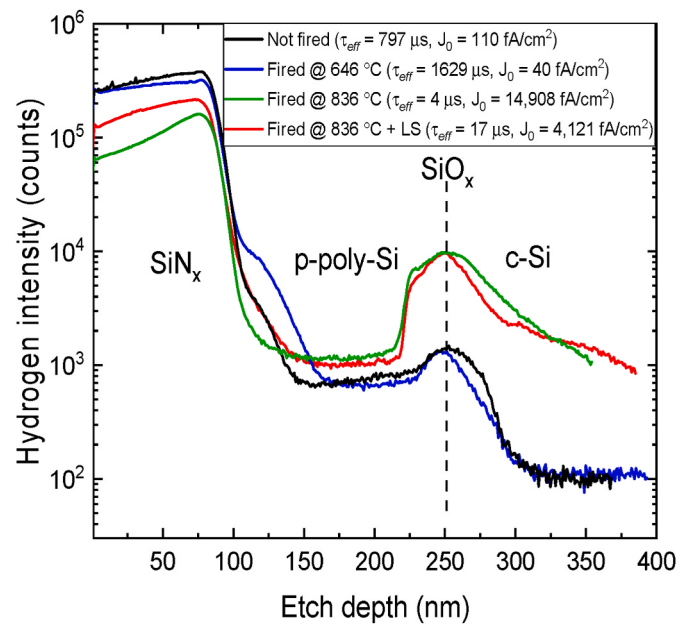
Fig. 8. Hydrogen ToF-SIMS profiles in unfired (black), fired at 646\ ^\circ\text{C} (blue), fired at 836\ ^\circ\text{C} (green) and fired at 836\ ^\circ\text{C} + light-soaked (red) p-type poly samples as a function of etch depth. The fired + LS (light-soaked) sample was analysed (along with other samples) after \sim 17 days of light soaking. All samples have a \text{SiN}_x coating.
