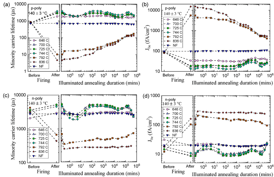
Fig. 7. (a) \tau_{eff} (p-poly) and (b) J_0 s (p-poly), and similarly (c) \tau_{eff} (n-poly) and (d) J_0 s (n-poly) during illuminated annealing at 1-sun and 140 °C. \tau_{eff} was extracted at \Delta n = 2 \times 10^{15}/\text{cm}^3 . NF refers to “non-fired” samples.
