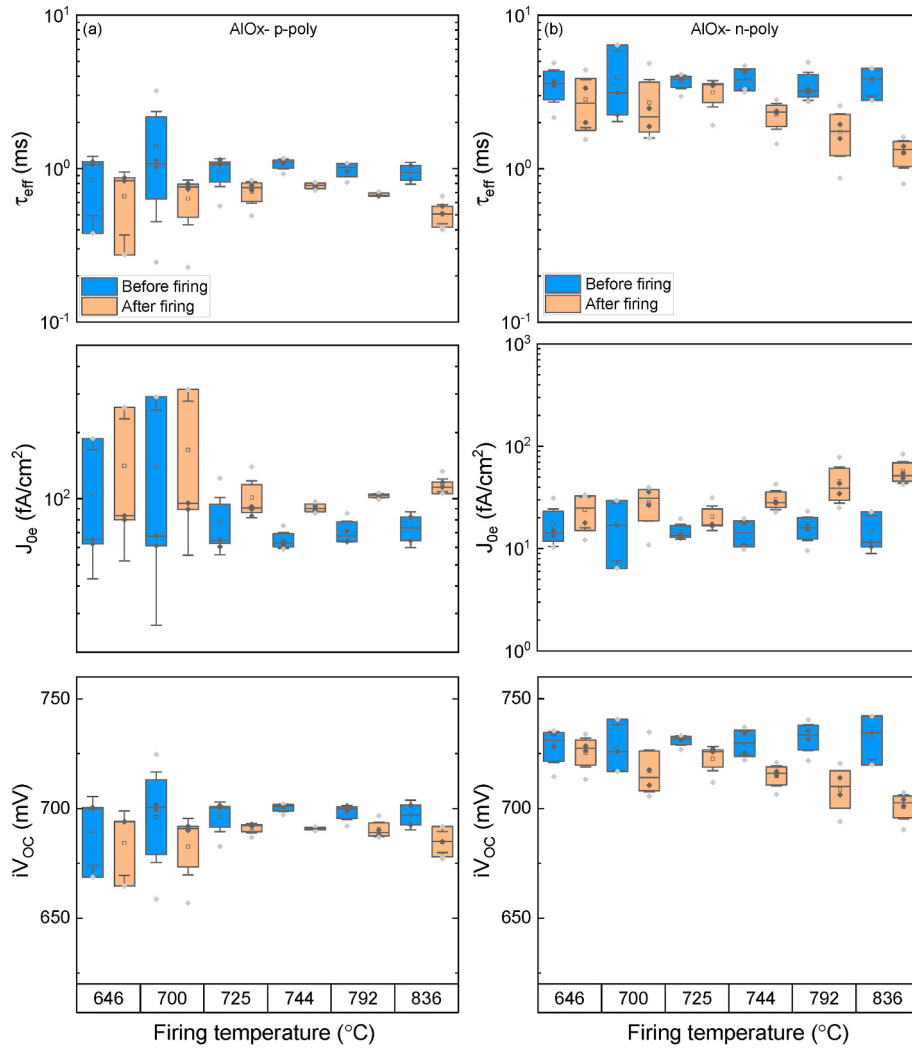
Fig. 1. \tau_{eff} (extracted at \Delta n = 2 \times 15/\text{cm}^3 ), J_0 and iV_{OC} before and after belt furnace firing at various temperatures for symmetrical \text{AlO}_x -capped (a) p-poly samples, and (b) n-poly samples.
