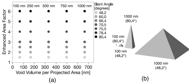
Fig. 11. (a) EAF versus VPA for the 35 nanopillar FDTD simulation conditions with the corresponding heights (vertical groups) and slant angles indicated. (b) Schematics of some unit cells (without substrate), shown on the same scale, with heights and slant angles indicated.
