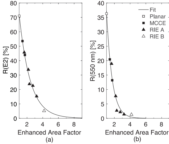
Fig. 5. (a) R(E2) and (b) R(550 nm) versus EAF for all texture conditions. Exponential decay fits to the data also shown.
