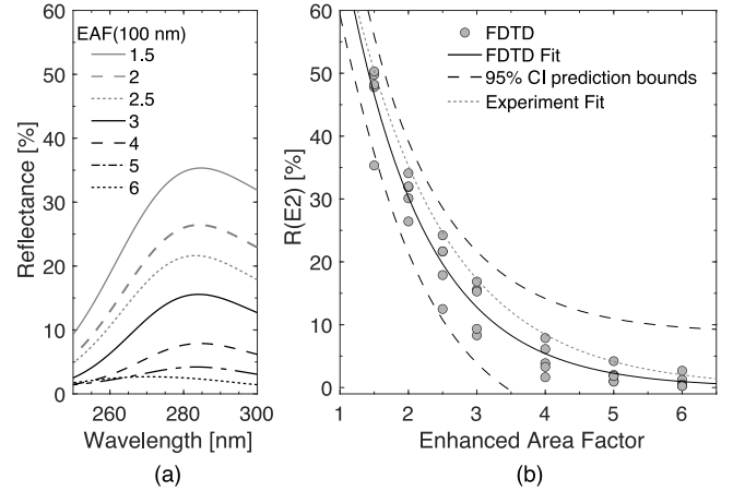
Fig. 12. (a) Simulated R(E2) peaks for the nanopillar conditions with 100 nm heights. (b) R(E2) peak values versus EAF for all the simulated conditions along with an exponential fit and 95% CI prediction bounds. The fit to the experimental data from Fig. 5 is also shown for reference.
