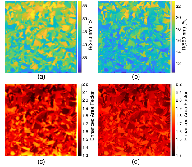
Fig. 6. (a) R(280 nm) map and (b) R(550 nm) map (154.75 mm by 154.75 mm) of a multicrystalline wafer with MCCE-M2 texture. The corresponding EAF maps calculated using the correlation fits from Fig. 5 are shown in (c) and (d).
